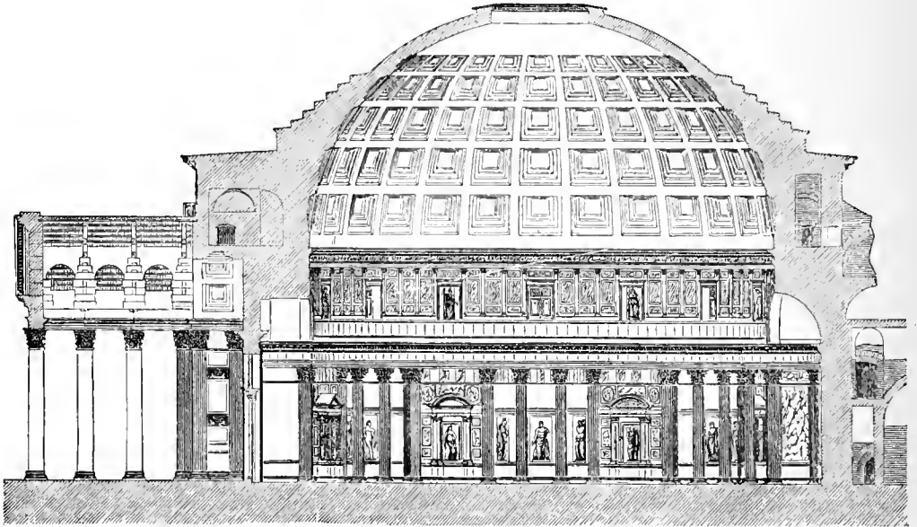
FIG. 137.—THE PANTHEON, ROME. INTERIOR.
